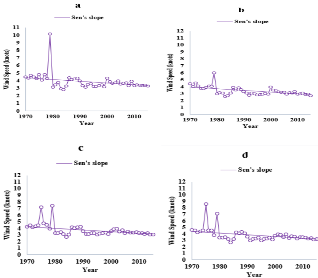
Figure 9. Variation of wind speed over the four-crop growing seasons (a) Aus, (b) Aman, (c) Boro and (d) Wheat, Sylhet, Bangladesh (1970-2018).
